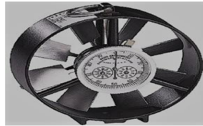
Illustration of (Back) of Anemometer Illustration of Dial Side (Front) of Anemometer
