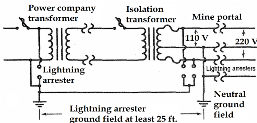
Figure 8: Acceptable lightning arresters for single-phase circuits. This circuit, with an isolation transformer installed, is acceptable since the neutral and lightning arrester grounds are separated by at least 25 feet.
