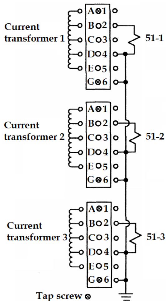
Figure 22: Terminals D and G are connected together and to one side of the relay coils. Terminal B is connected to the other side of the relay coils. However, the tap screws short A to G and thus effectively short out the current transformer secondaries.
