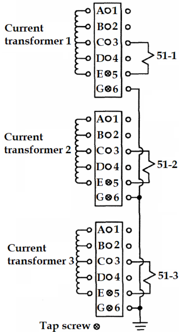
Figure 20: Terminals C and E are connected to the relay coils. From the table, the ratio of primary to secondary current in the transformers is 90/1. Notice that the tap screws short E to G, which effectively grounds one side of the transformer secondaries.
