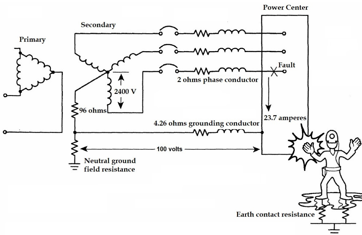
Figure 1: Touch potential of a resistance grounded system under fault conditions (refer to Appendix F for calculations).
