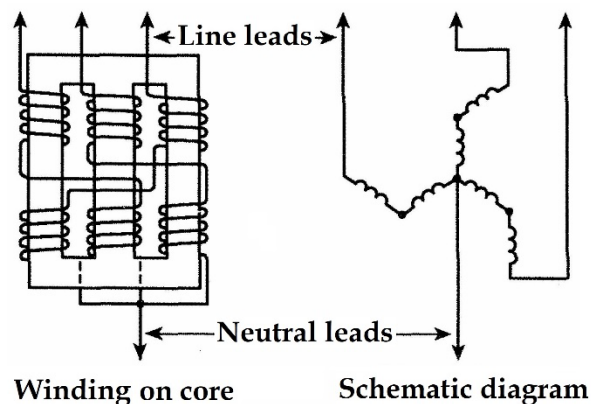
Figure 3: Zigzag three-phase grounding transformer.
