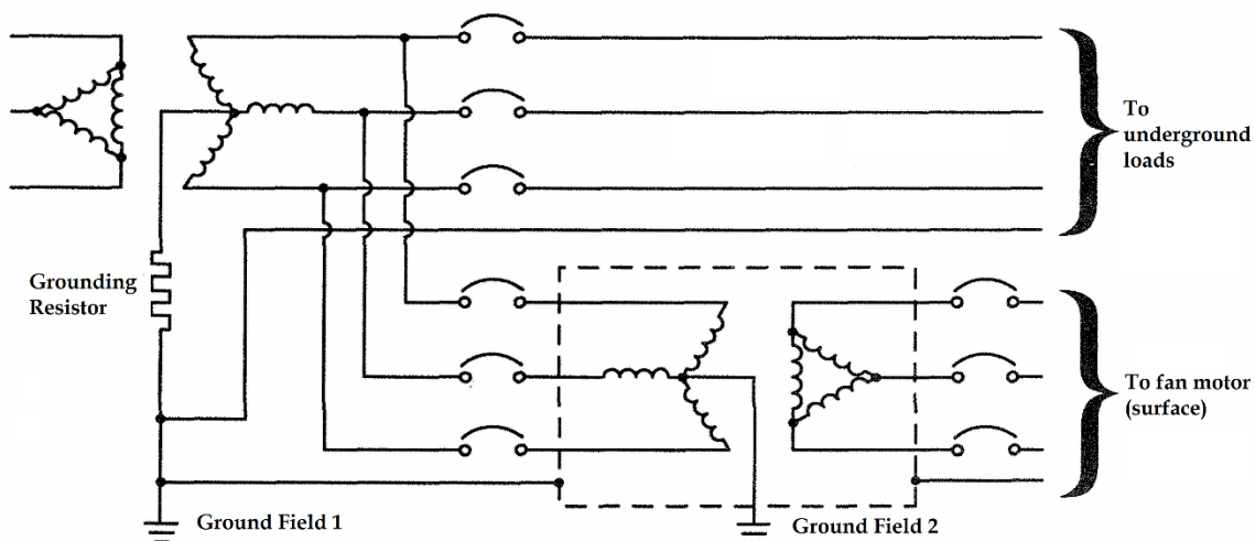
Figure 5: An unacceptable ground fault configuration. This system will not comply since fault current will flow through the second neutral (connected to ground field 2), effectively shorting out the grounding resistor during fault conditions.
