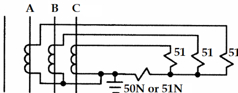
Figure 15: Residual trip relaying to provide grounded-phase protection.
