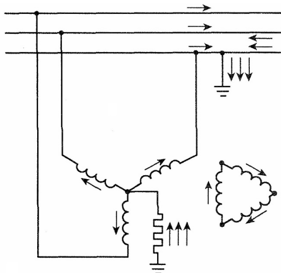
Figure 5: An unacceptable ground fault configuration. This system will not comply since fault current will flow through the second neutral (connected to ground field 2), effectively shorting out the grounding resistor during fault conditions.
