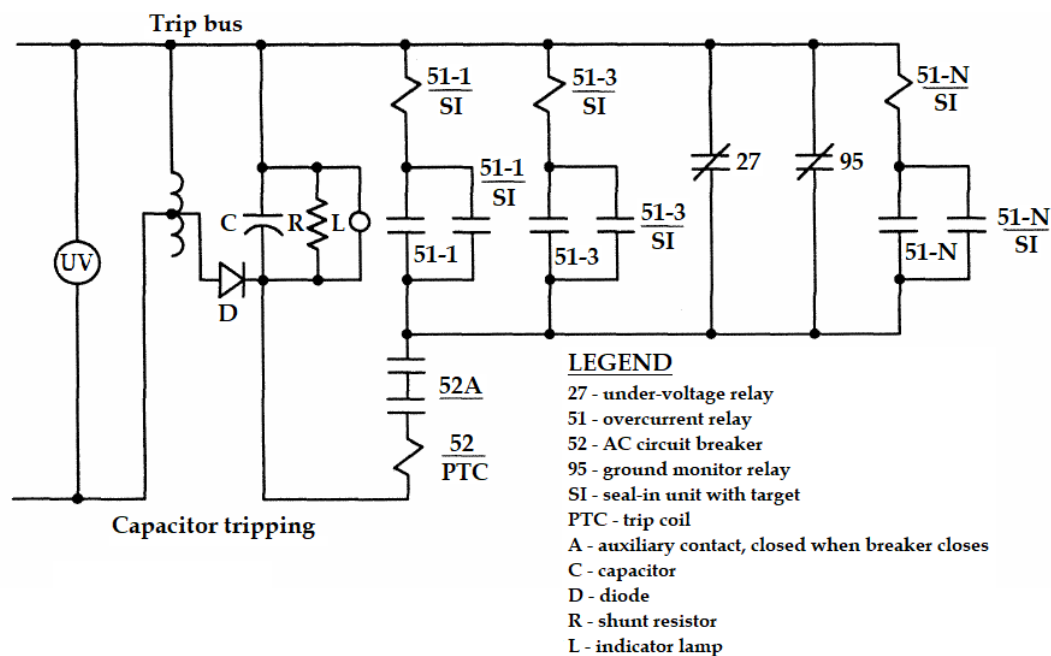
Figure 24: Typical AC control circuit for a high-voltage circuit breaker.
