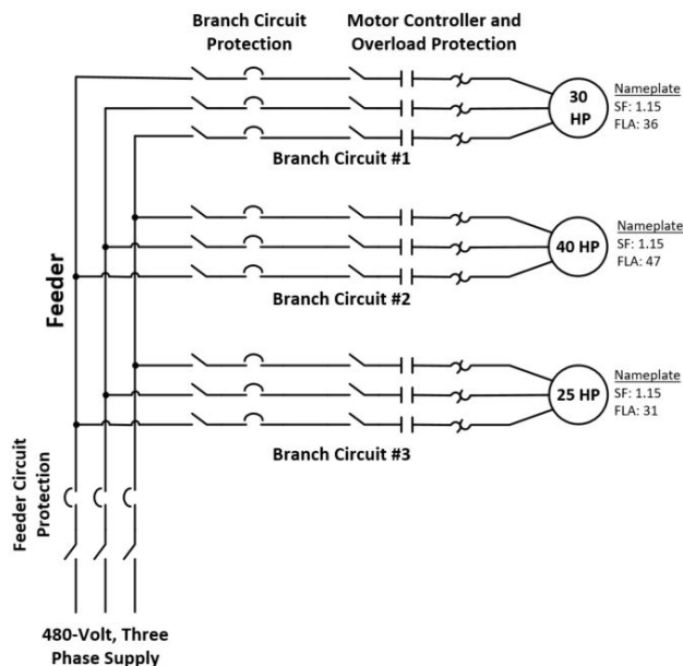
Figure 12 – Motor Circuit
