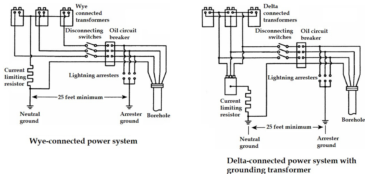
Figure 2: Properly connected resistance grounded circuits.
