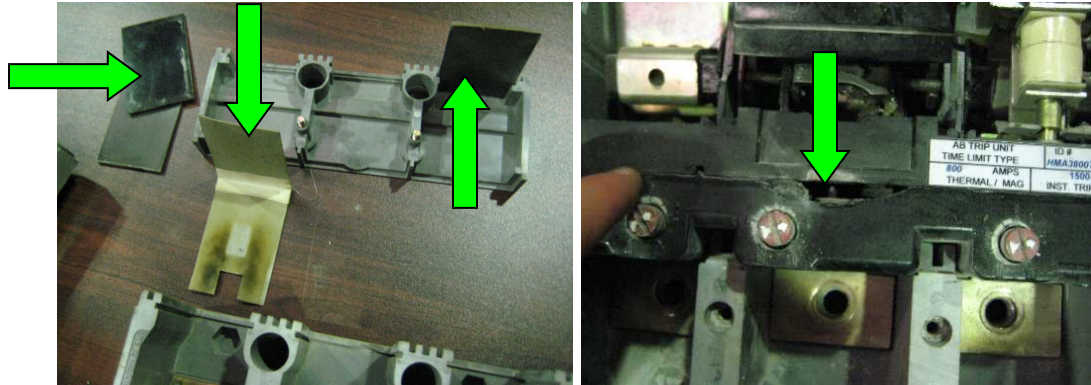
Fish Boards
