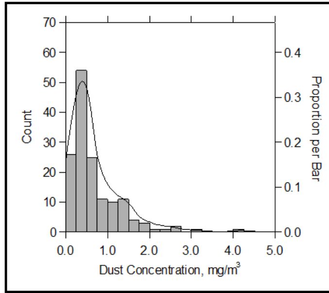
Figure 32. — Example “B”: a WL where the frequency distribution of respirable coal mine dust concentrations diverges significantly from a lognormal model.
