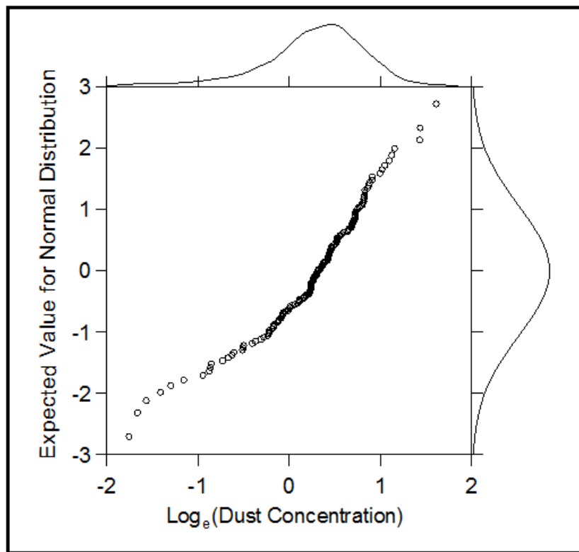
Figure 37. — Lognormal probability plot for the respirable coal mine dust concentrations measured on 150 different shifts at WL “D.” Divergence from lognormal distribution is indicated by deviation of points from a straight line.
