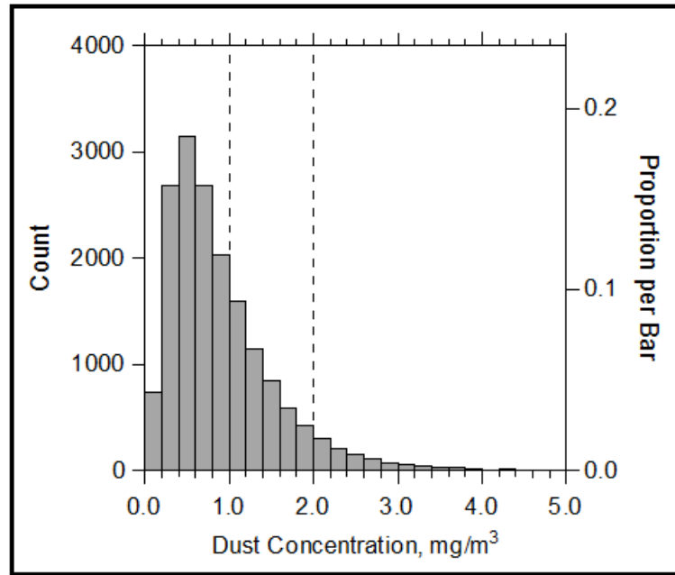
Figure 3. — Respirable coal mine dust concentration distribution for continuous miner operators, based on 17,065 MSHA inspector samples collected from 2004-2008. 33 measurements exceeding 5.0 mg/m 3 are excluded. Vertical dashed lines are plotted at 1.0 mg/m 3 and 2.0 mg/m 3 .
