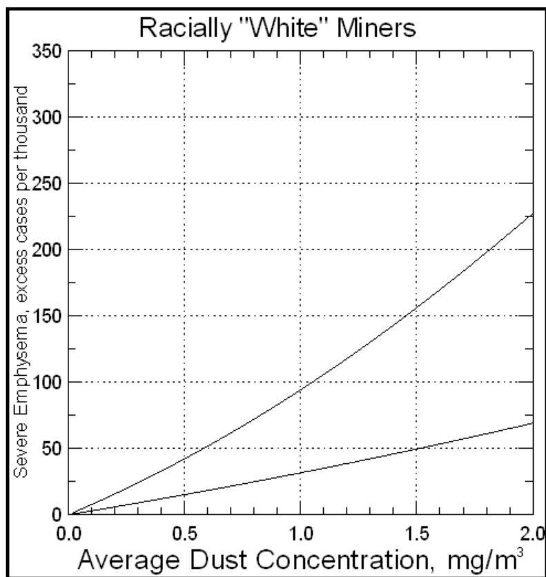
Figure 23. — 90-percent confidence band for excess risk of emphysema for never-smoking white miners at age 73 after 45 years of occupational exposure to RCMD.
