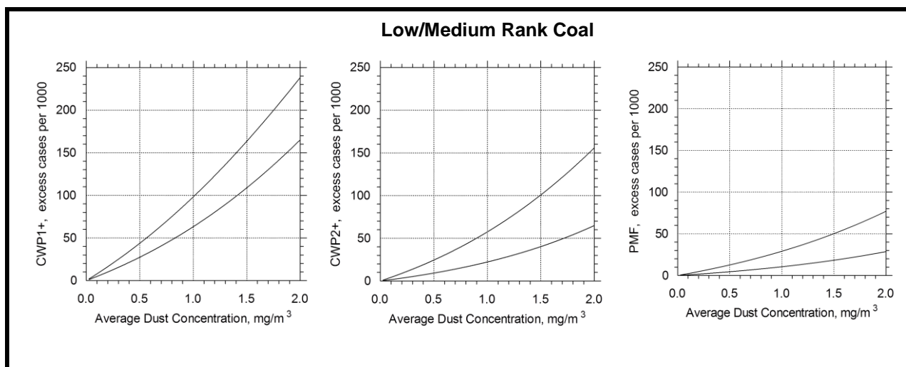
Figure 10. — Estimated relationship between average respirable coal mine dust concentration experienced over a 45-year working lifetime and excess risk of CWP1+, CWP2+, and PMF for workers at low and medium rank U.S. bituminous coal mines. Upper and lower curves are for 73 and 65 year-old miners, respectively.
