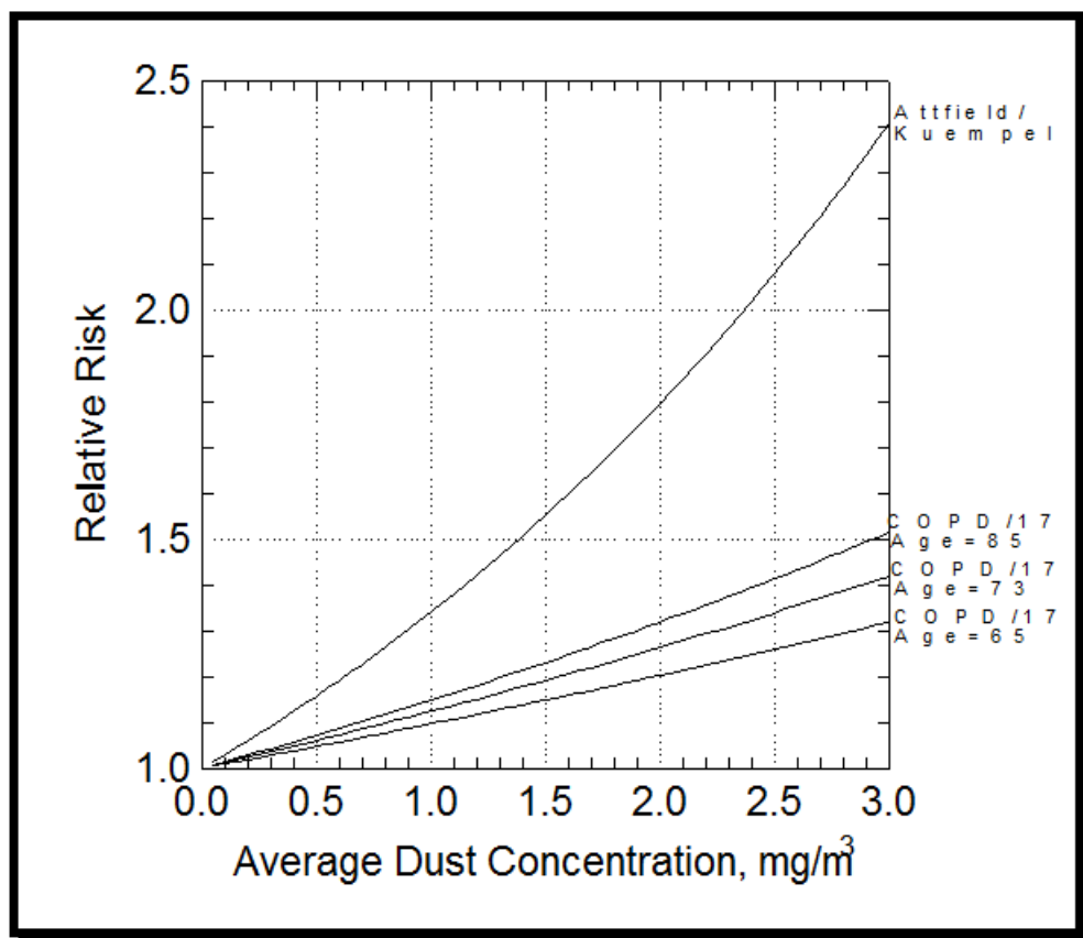
Figure 15. — Estimated relationship between average coal mine dust concentration experienced over a 45-year working lifetime and Relative Risk for death due to COPD. Attfield/Kuempel model is based on cohort mortality among U.S. coalminers and relates to un-lagged cumulative dust exposure. COPD/17 model is based on cohort mortality among British coalminers and relates to cumulative dust exposure lagged by 15 years.
