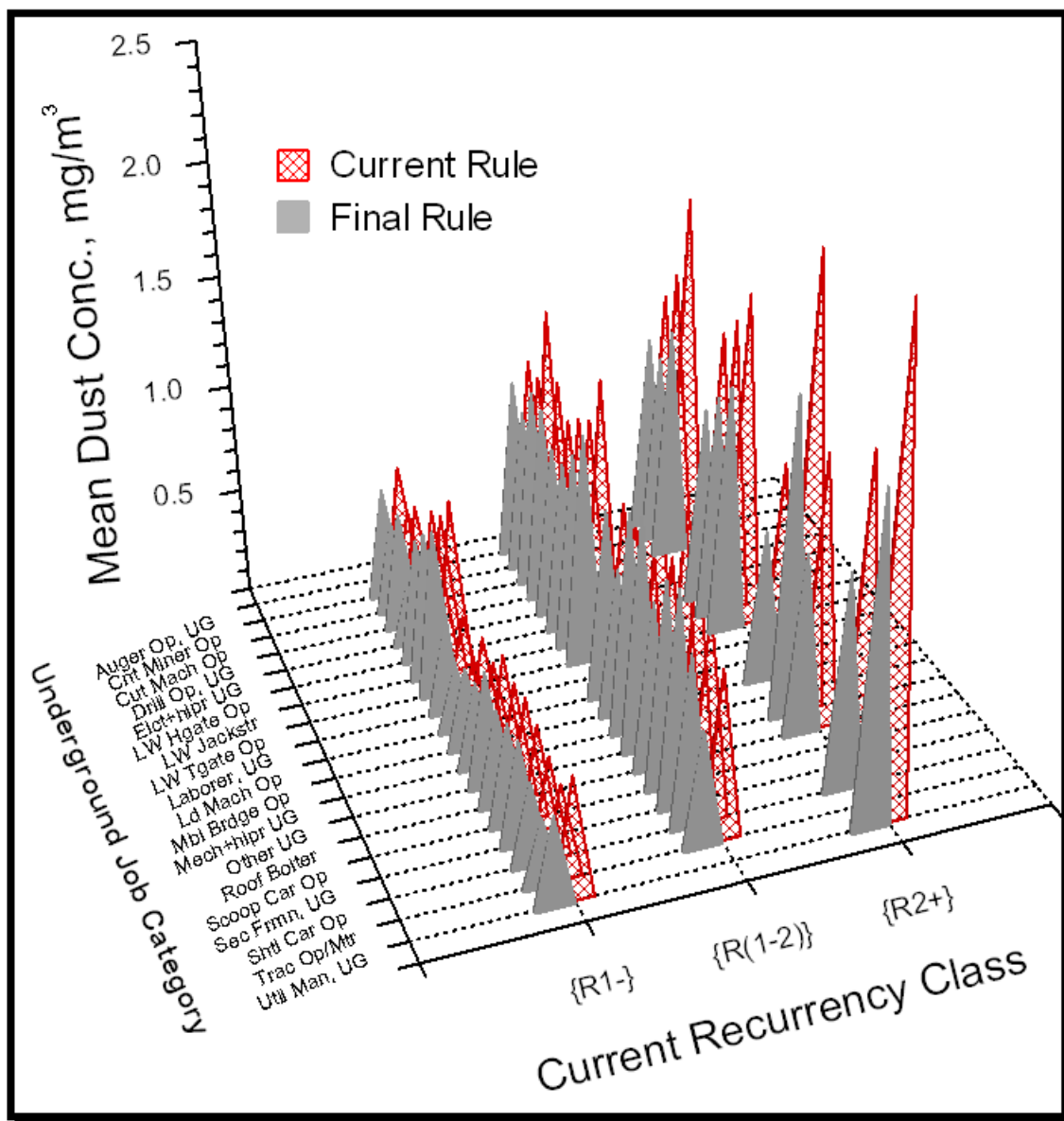
Figure 18. — Comparison of current and projected underground coal mine dust concentrations, by job-category and current recurrency class.
