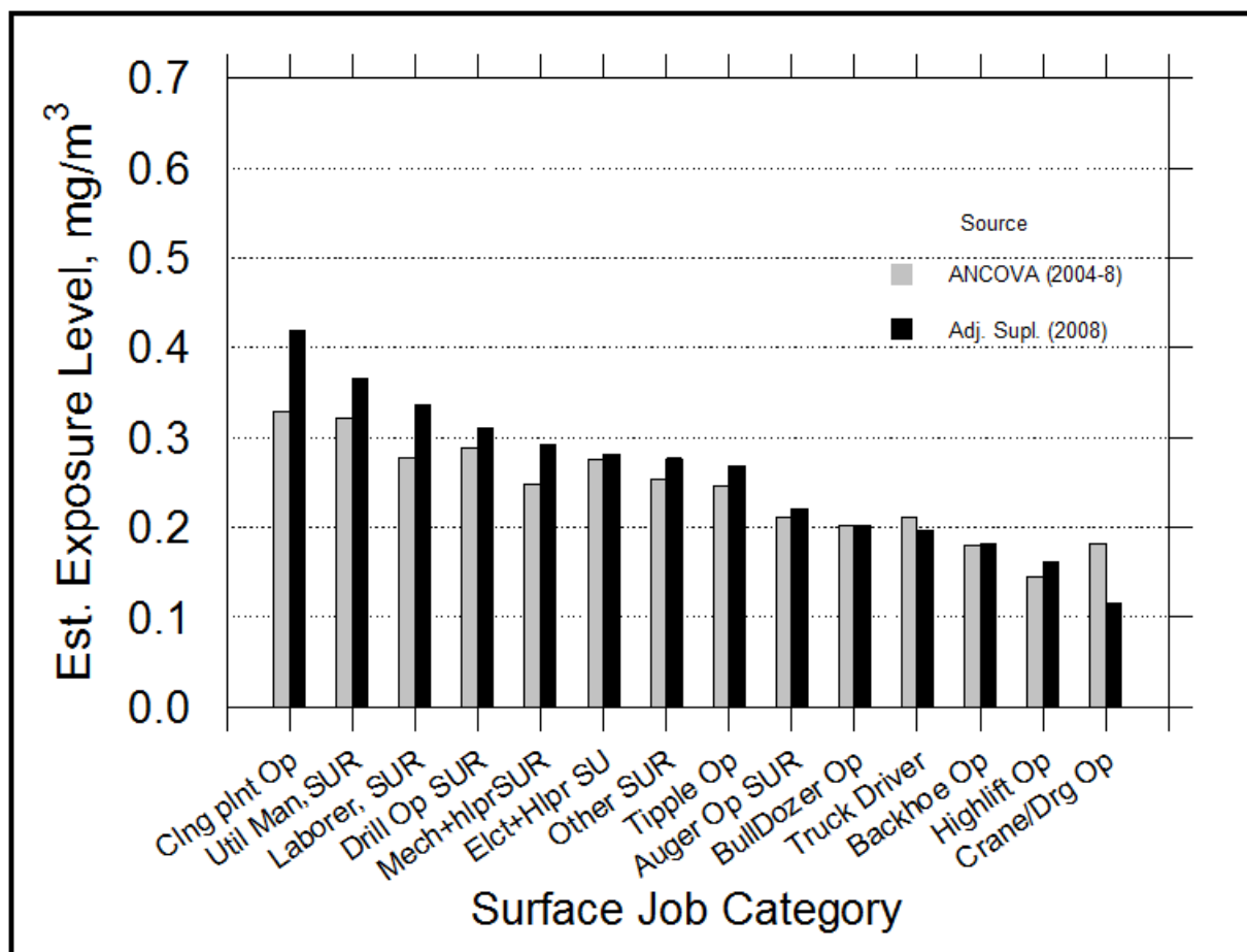
Figure 9. — Surface respirable dust exposure levels aggregated by occupation, as estimated from ANCOVA (2004–2008 MSHA inspector data) or from Adjusted and Supplemented (AS) estimation procedure (2008 MSHA inspector data supplemented by 2008 mine operator data). Health risks in this QRA are evaluated based on the AS estimates.
