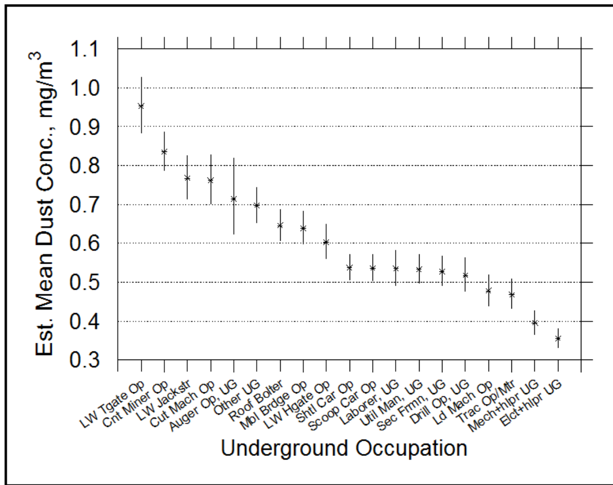
Figure 7. — Estimated mean respirable coal mine dust concentration for underground occupations on shifts sampled by MSHA from 2004–2008. Estimates are adjusted to correct for unbalanced factors at different sampling locations. Vertical line approximates 95-percent confidence interval for the estimated mean.
