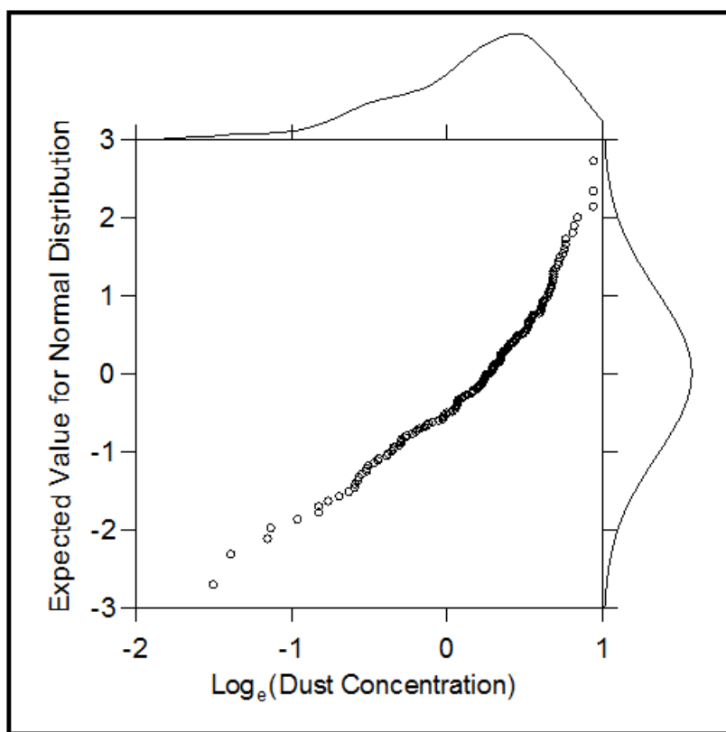
Figure 35. — Lognormal probability plot for the respirable coal mine dust concentrations measured on 150 different shifts at WL “C.” Divergence from lognormal distribution is indicated by deviation of points from a straight line.
