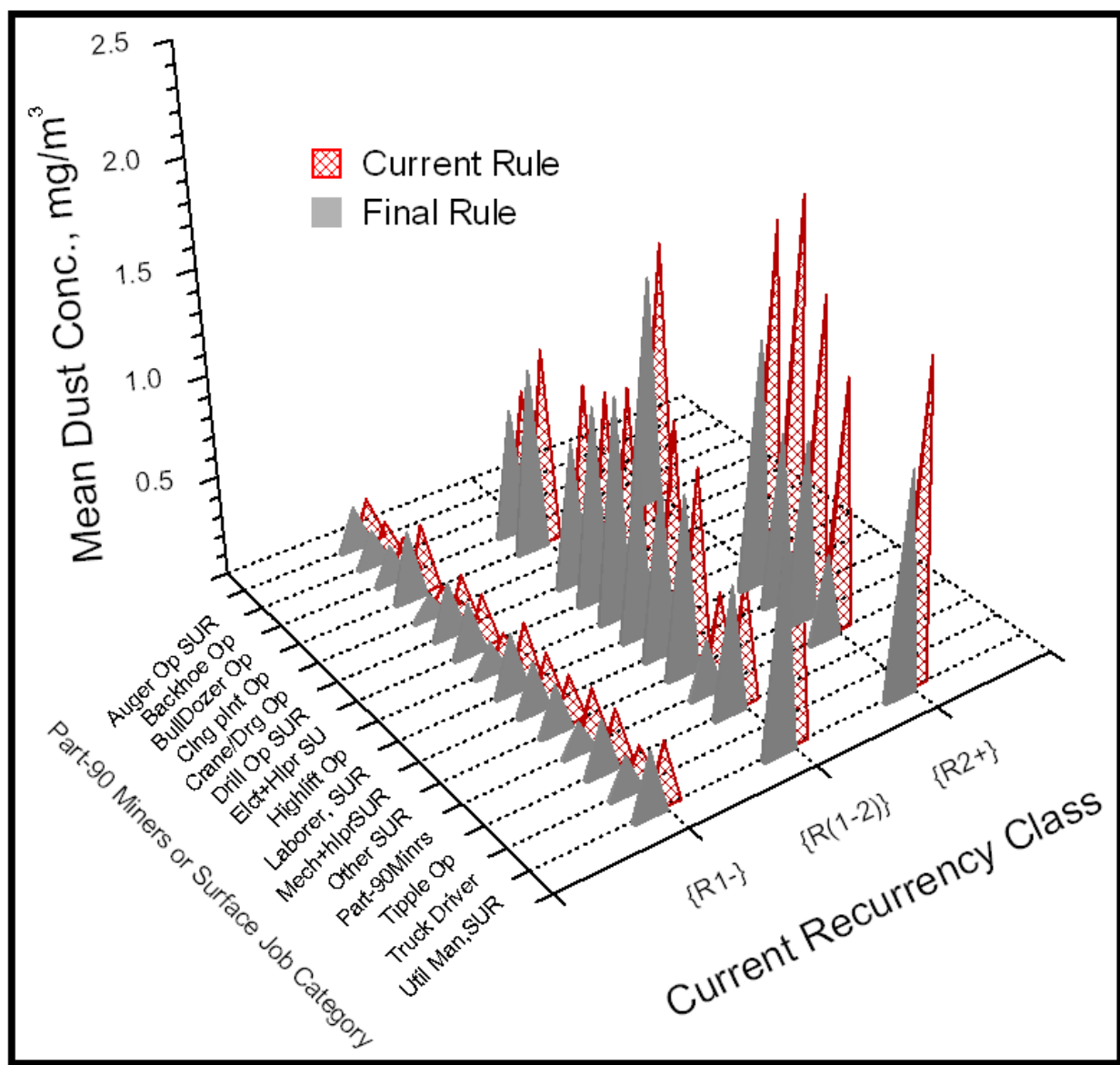
Figure 19. — Comparison of current and projected coal mine dust concentrations for Part 90 miners and surface occupations, by job-category and current recurrency class.
