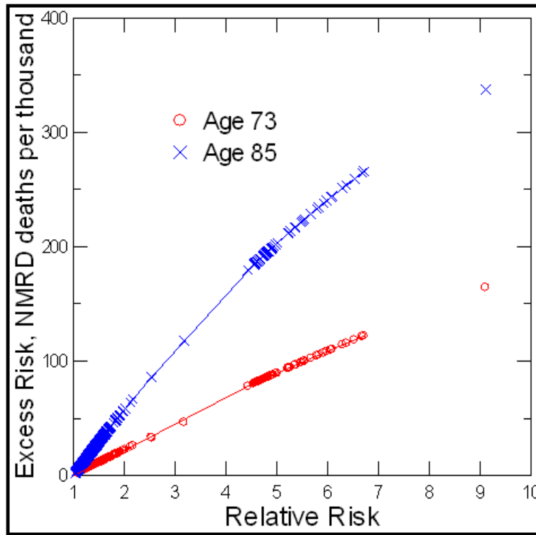
Figure 42. — Relationship between relative and excess risks of NMRD mortality at ages 73 and 85 years.
