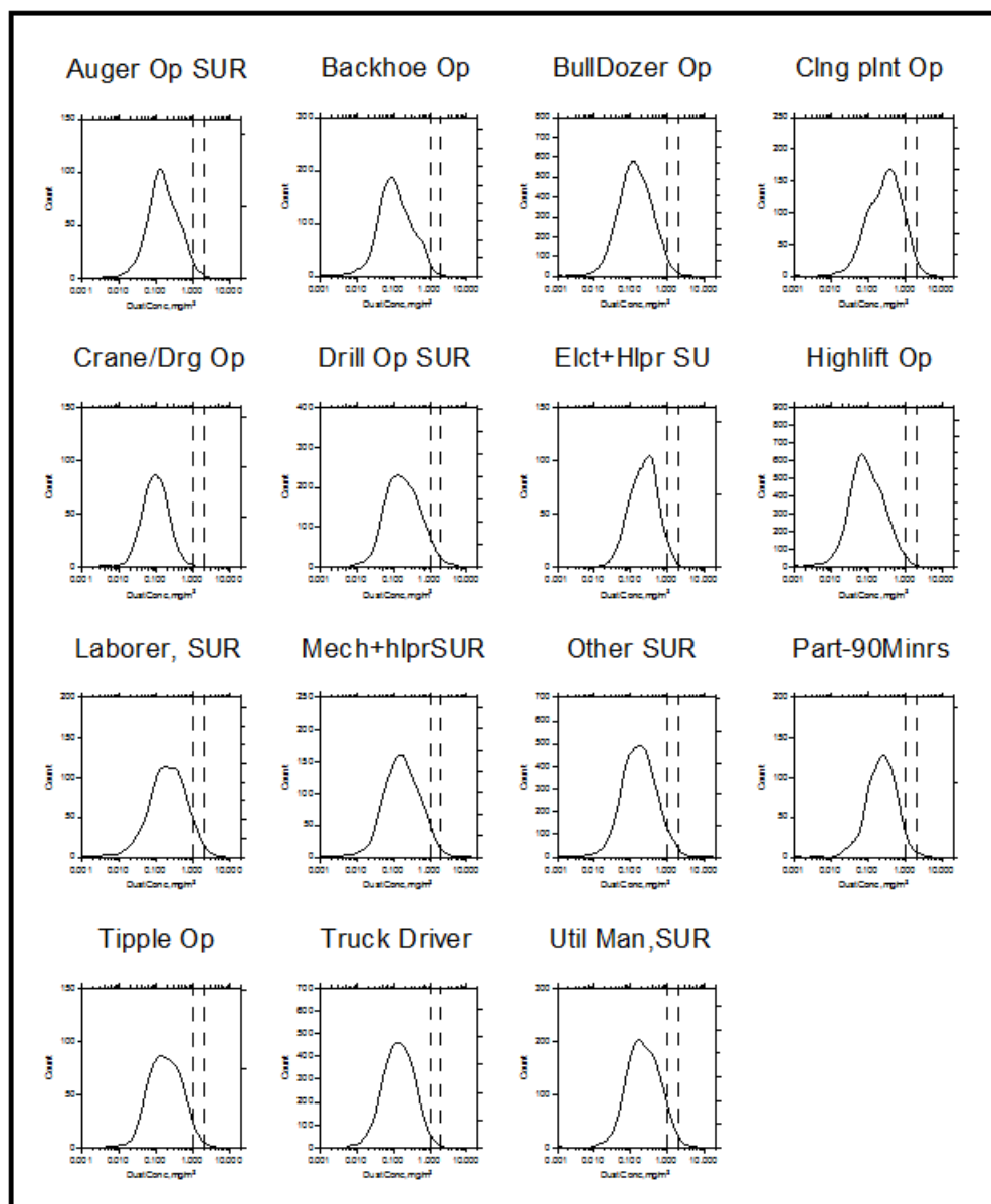
Figure 27. — Frequency distributions of Part 90 miners and surface respirable coal mine dust concentrations measured by MSHA inspectors, 2004-2008, plotted on a logarithmic scale by job category. Vertical dashed lines are plotted at 1.0 mg/m 3 and 2.0 mg/m 3 .
