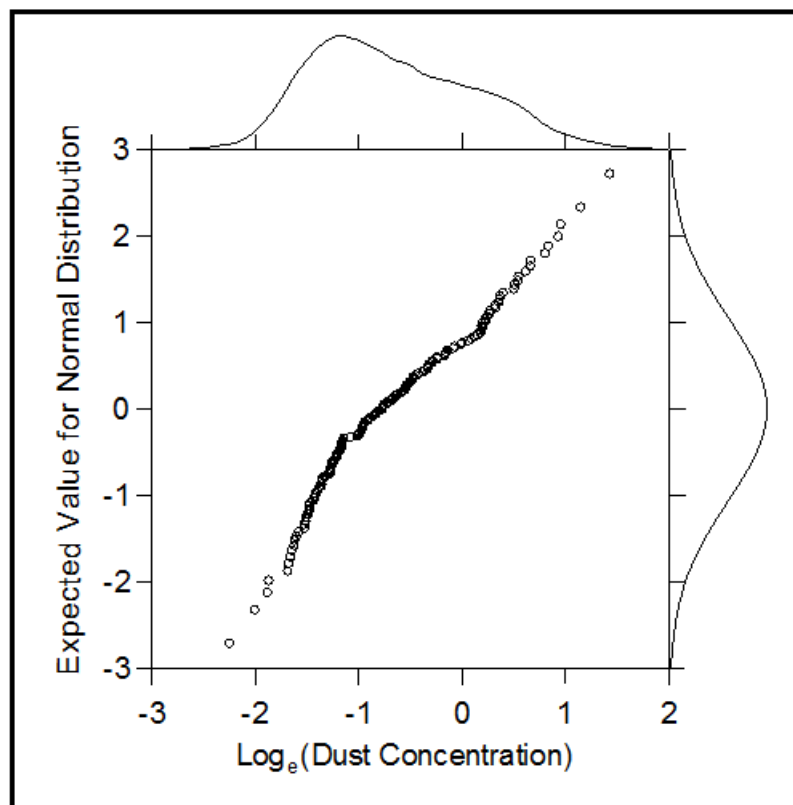
Figure 33. — Lognormal probability plot for the respirable coal mine dust concentrations measured on 150 different shifts at WL “B.” Divergence from lognormal distribution is indicated by deviation of points from a straight line.
