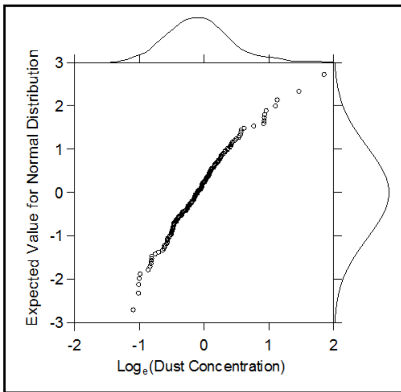
Figure 31. — Lognormal probability plot for the respirable coal mine dust concentrations measured on 150 different shifts at WL “A.” Validity of lognormal approximation is indicated by points’ falling approximately along a straight line.
