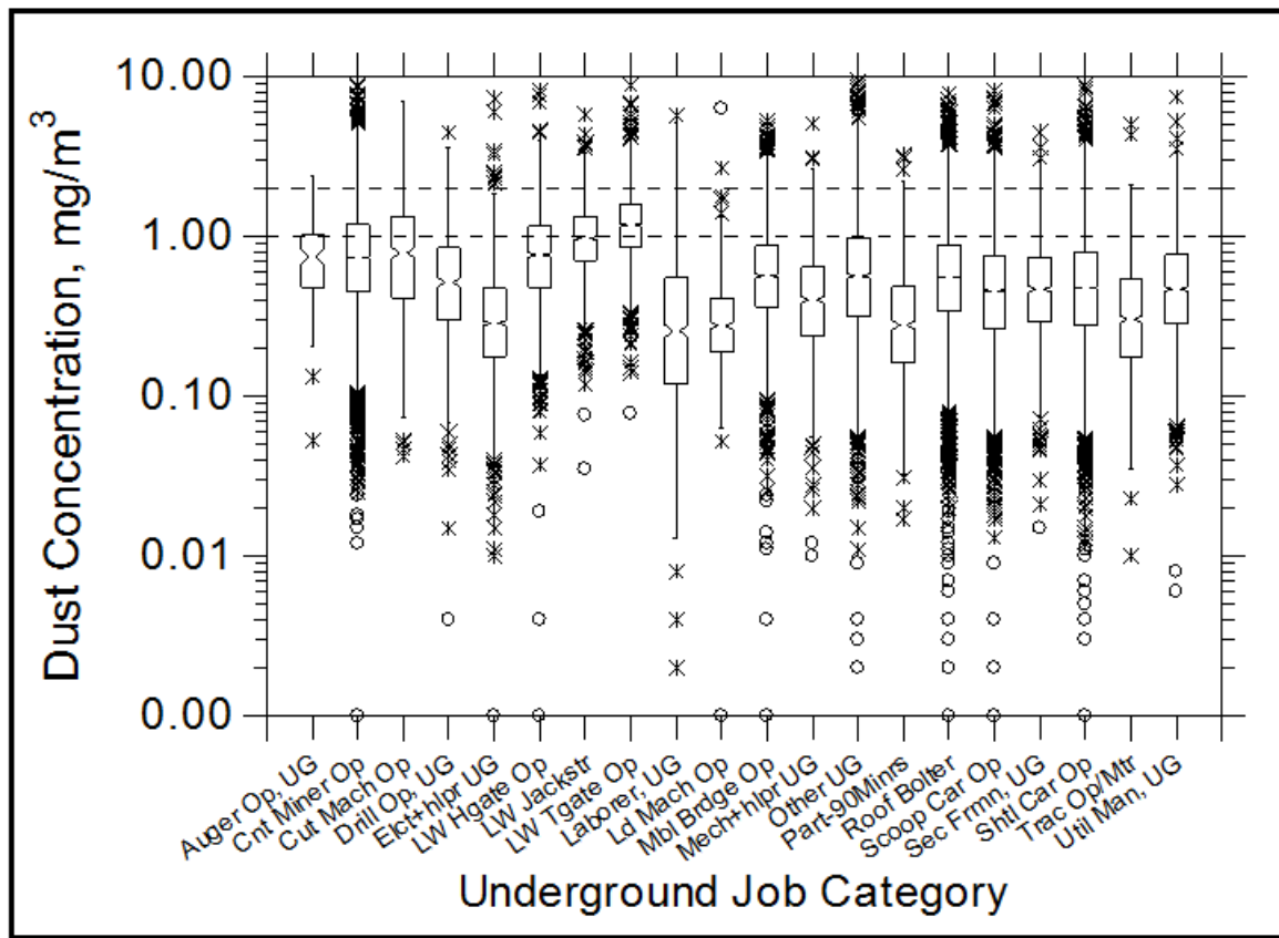
Figure 1. — Box Plots (Tukey, 1977) for coal mine dust concentrations measured by MSHA inspectors, 2004-2008, on selected underground occupations. Top and bottom of each box represent upper and lower quartiles, respectively. Notch within each box represents 95-percent confidence interval for the median. Vertical lines span most measurements. Isolated points (either \circ or * ) are outliers, representing unusually low or high observations compared to other measurements for the same job category. Horizontal dashed lines are plotted at 1.0 \text{ mg/m}^3 and 2.0 \text{ mg/m}^3 .
