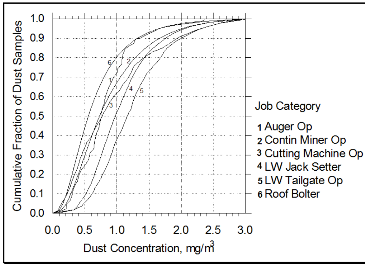
Figure 5. — Cumulative distribution of MSHA inspector coal mine dust measurements, 2004-2008, for selected underground occupations. Of 48,327 measurements for the listed occupations, 514 were excluded because they exceeded 3.0 mg/m 3 . Vertical dashed lines are plotted at 1.0 mg/m 3 and 2.0 mg/m 3 .
