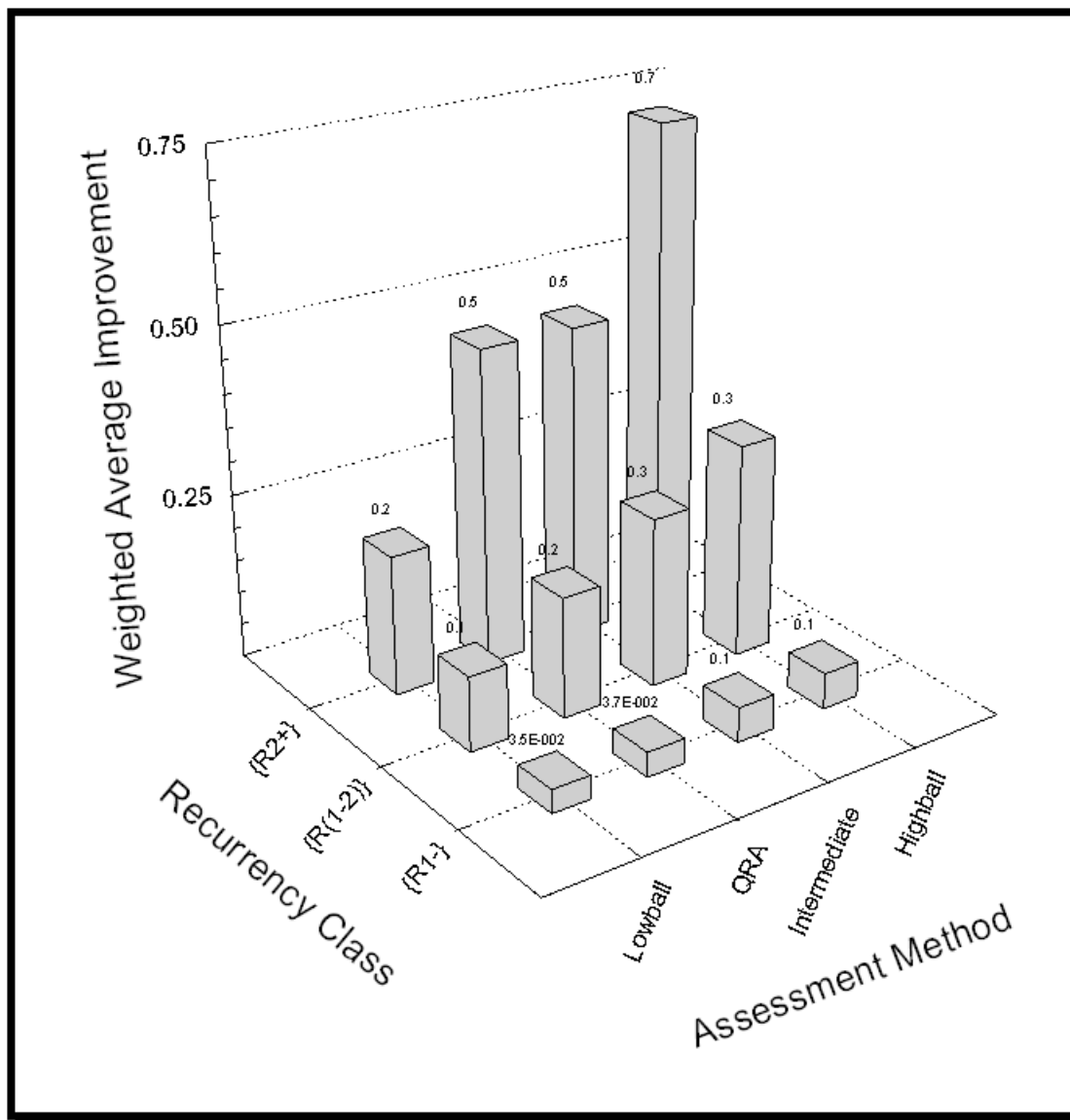
Figure 20. — Range of improvements in weighted average exposure ( \text{mg}/\text{m}^3 ) projected by four alternative assessment methods, broken out by current recurrency class.
