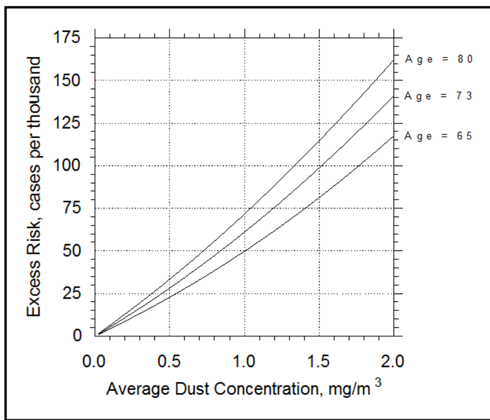
Figure 14. — Estimated relationship between average coal mine dust concentration experienced over a 45-year working lifetime and excess risk of developing emphysema severity corresponding to \text{FEV}_1 < 65\% of predicted normal value, for white, never-smoking U.S. coal miners at ages 65, 73, and 80 years.
