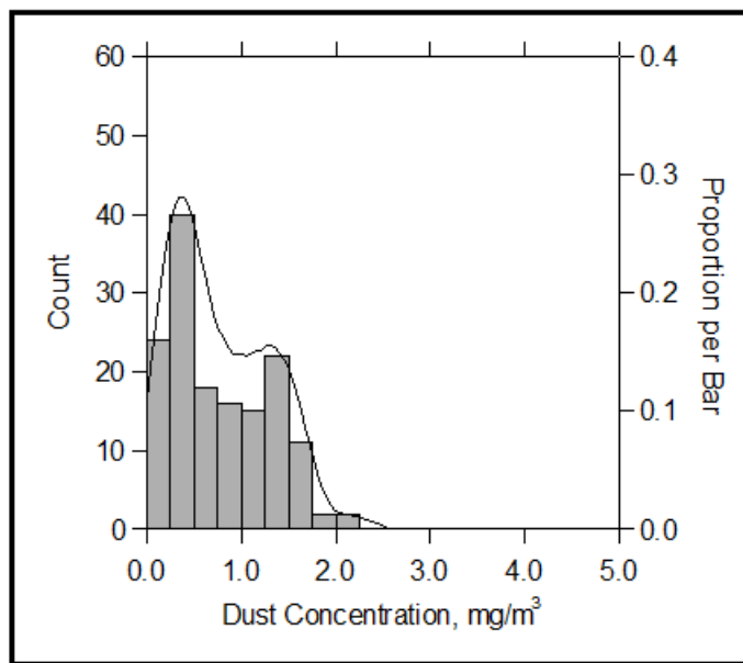
Figure 38. — Example “E”: a WL where the frequency distribution of respirable coal mine dust concentrations diverges significantly from a lognormal model.
