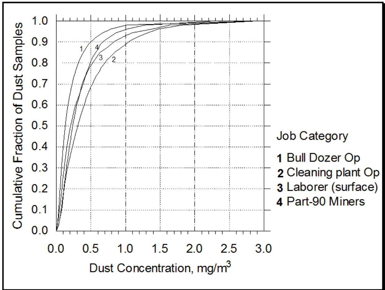
Figure 6. — Cumulative distribution of MSHA inspector coal mine dust measurements, 2004-2008, for Part 90 miners and selected surface occupations. Of 11,981 measurements for the listed categories, 25 were excluded because they exceeded 3.0 mg/m³. Vertical dashed lines are plotted at 1.0 mg/m³ and 2.0 mg/m³.
