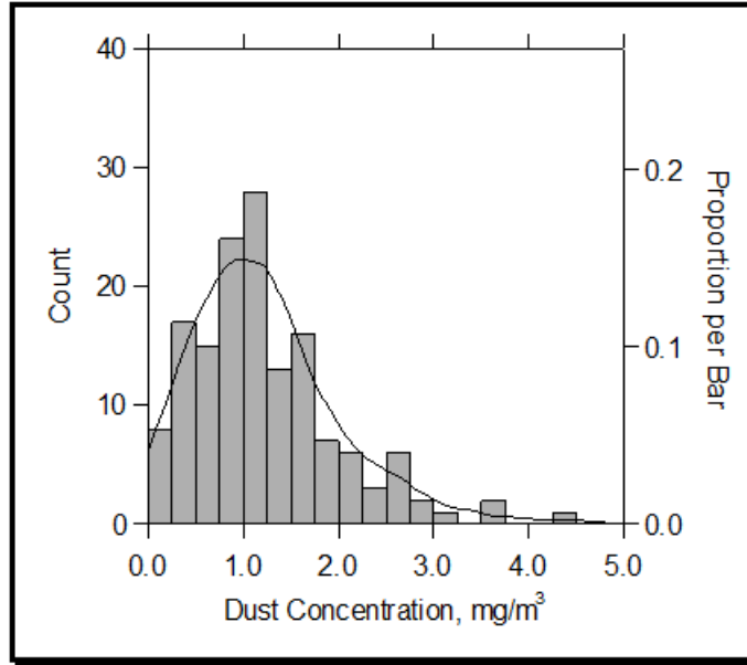
Figure 40. — Example “F”: a WL where the frequency distribution of respirable coal mine dust concentrations diverges significantly from a lognormal model. One measurement exceeding 5.0 mg/m 3 was excluded from the chart.
