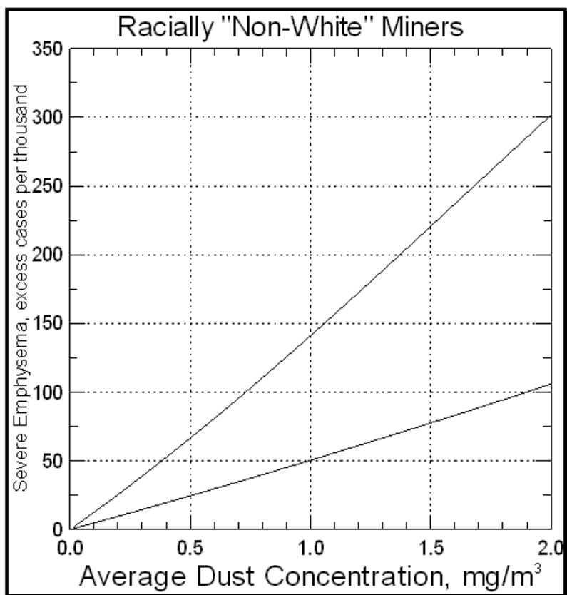
Figure 24. — 90-percent confidence band for excess risk of emphysema for never-smoking non-white miners at age 73 after 45 years of occupational exposure to RCMD.
