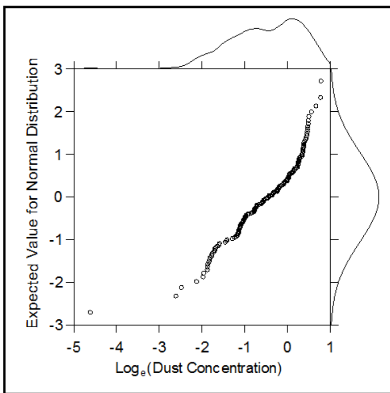
Figure 39. — Lognormal probability plot for the respirable coal mine dust concentrations measured on 150 different shifts at WL “E.” Divergence from lognormal distribution is indicated by deviation of points from a straight line.
