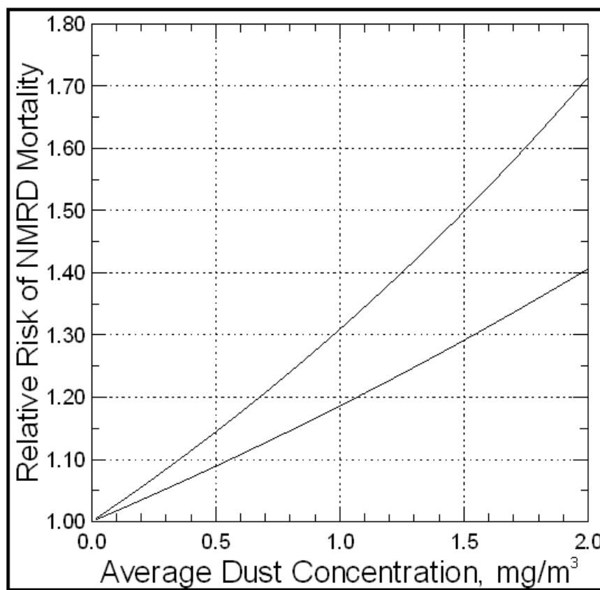
Figure 25. — 90-percent confidence band for relative risk (RR) of NMRD mortality after 45 years of occupational exposure to RCMD.
