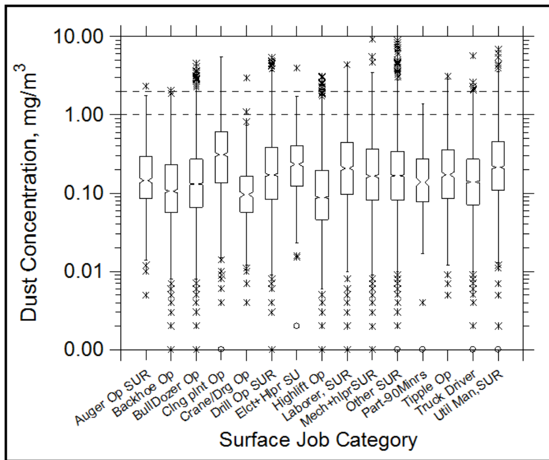
Figure 2. — Box Plots (Tukey, 1977) for coal mine dust concentrations measured by MSHA inspectors, 2004-2008, on selected surface occupations. Top and bottom of each box represent upper and lower quartiles, respectively. Notch within each box represents 95-percent confidence interval for the median. Vertical lines span most measurements. Isolated points (either \circ or * ) are outliers, representing unusually low or high observations compared to other measurements for the same job category. Horizontal dashed lines are plotted at 1.0 \text{ mg/m}^3 and 2.0 \text{ mg/m}^3 .
