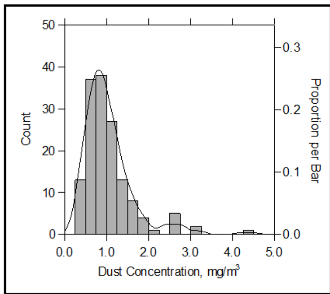
Figure 30. — Example “A”: a WL where the frequency distribution of respirable coal mine dust concentrations can be adequately modeled as being lognormal. One measurement exceeding 5.0 mg/m 3 was excluded from chart.
