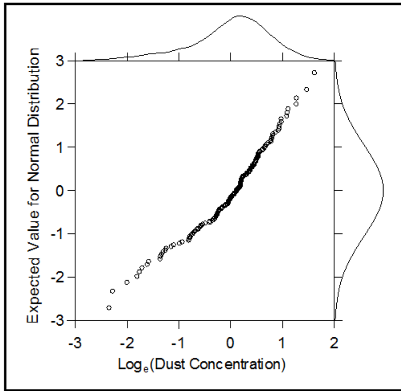
Figure 41. — Lognormal probability plot for the respirable coal mine dust concentrations measured on 150 different shifts at WL “F.” Divergence from lognormal distribution is indicated by deviation of points from a straight line.
