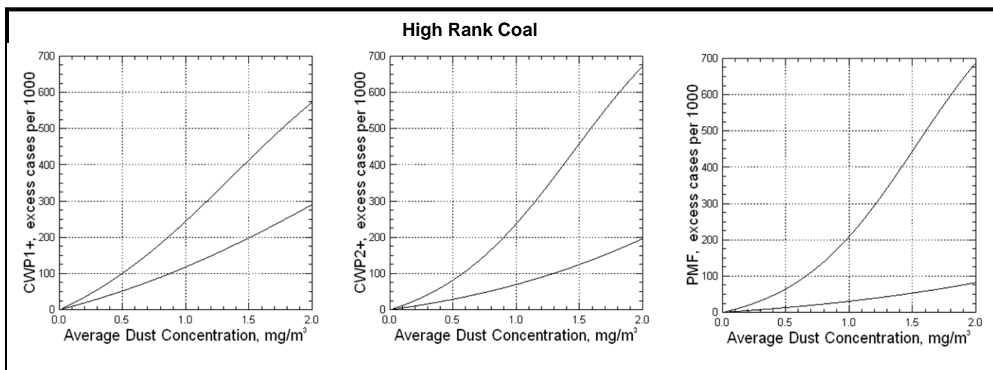
Figure 22. — 90-percent confidence bands for excess risk of CWP1+, CWP2+, and PMF at age 73 after 45 years of occupational exposure to RCMD at high rank coal mines.
