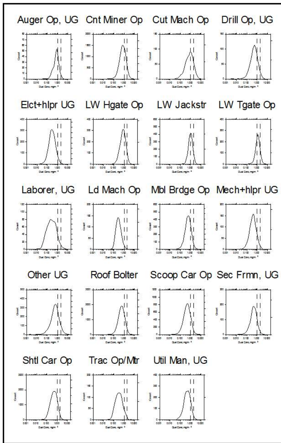
Figure 26. — Frequency distributions of underground respirable coal mine dust concentrations measured by MSHA inspectors, 2004-2008, plotted on a logarithmic scale by job category. Vertical dashed lines are plotted at 1.0 mg/m 3 and 2.0 mg/m 3 .
