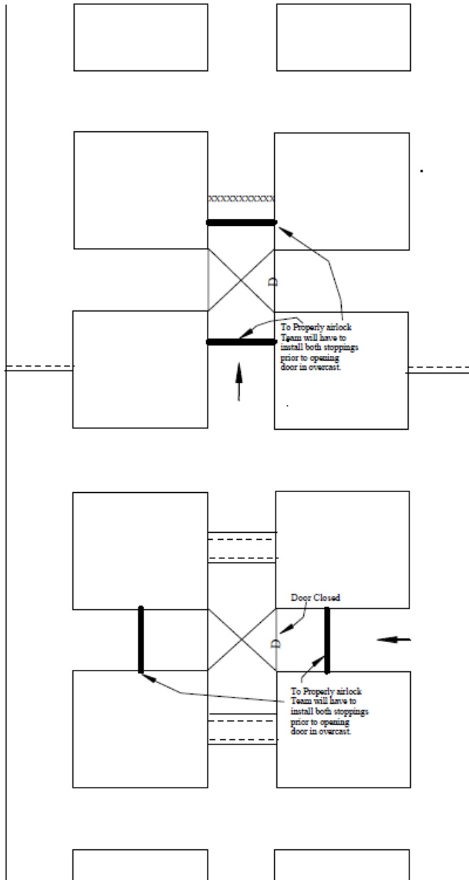
Figure 6 Airlocking Through an Overcast Wall
