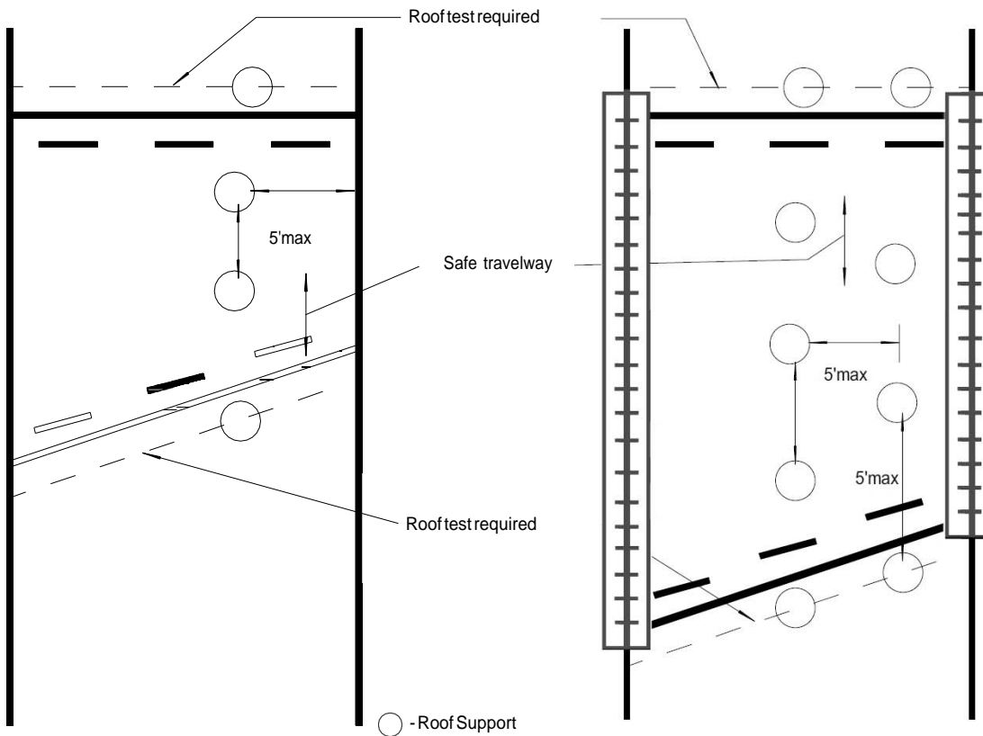
Figure 2 EXAMPLES OF PROPER METHODS OF SETTING ROOF SUPPORTS
